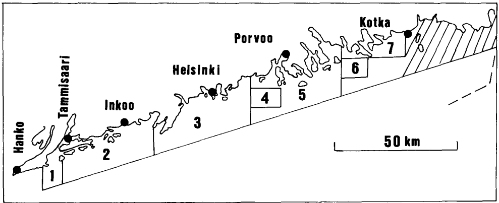
FIG. 1. The study area and the subareas from which data were collected (see text and Table 1 for further details). The data from the hatched area are still scanty.
