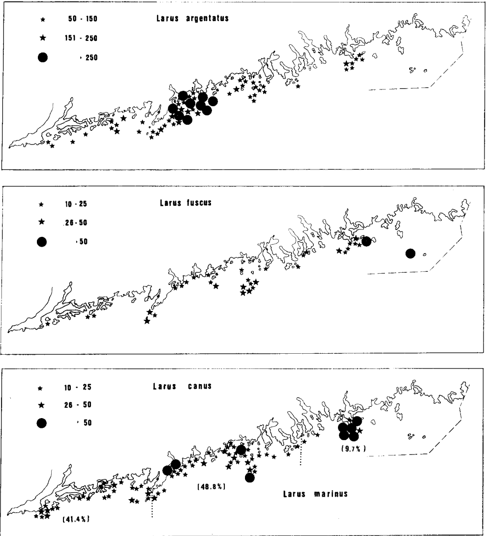
FIG. 2. The known main colonies of Larus argentatus (top), L. fuscus (middle) and L. canus (bottom). The numbers of L. marinus are presented as percentages of the total number (N = 360) for three segments of the coast (bottom).
